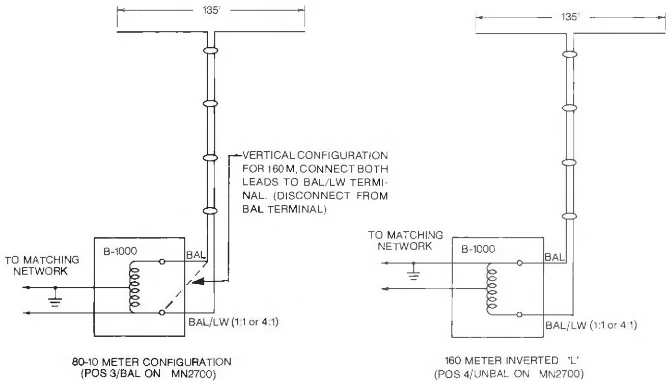
Fig. 3-3 Multiband Antenna Configurations
