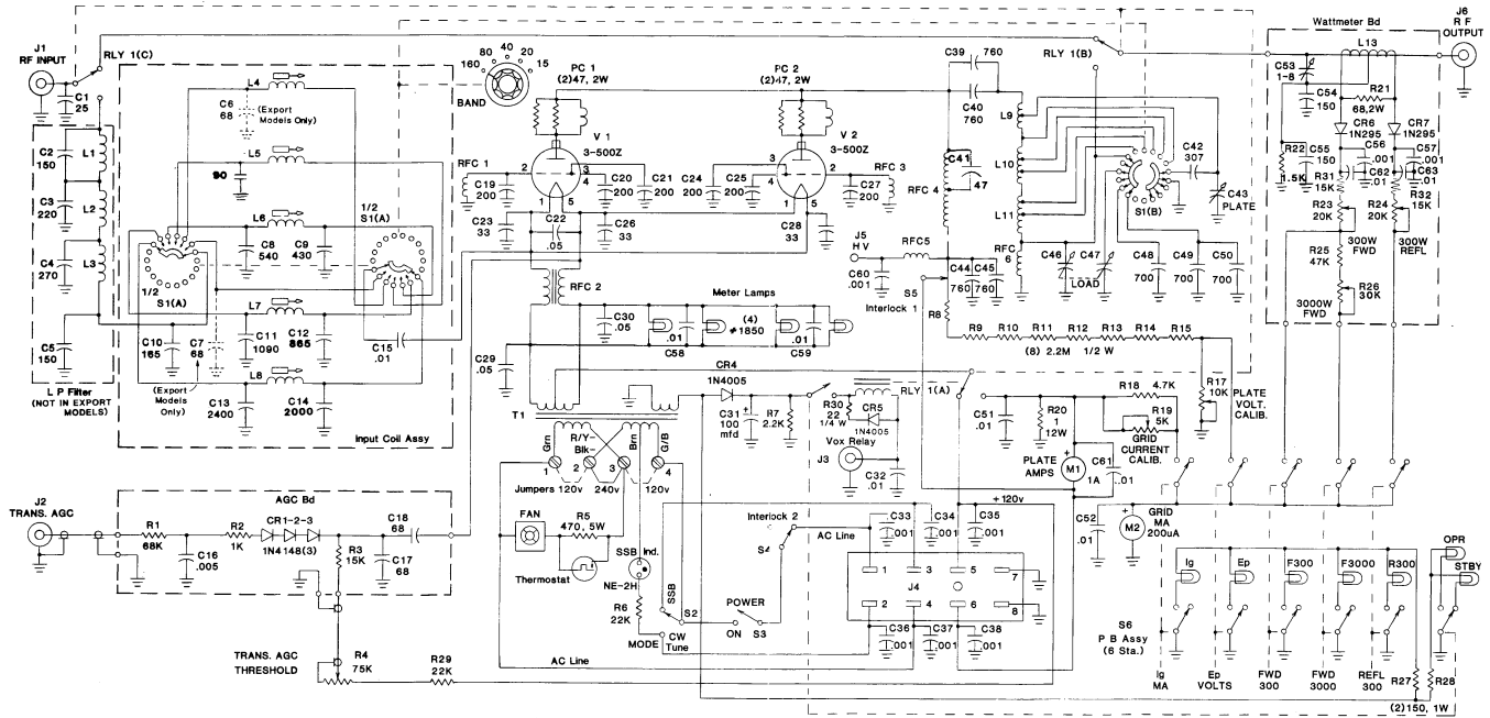
Fig. 5-5 Model L7 Linear Amplifier Schematic Diagram
