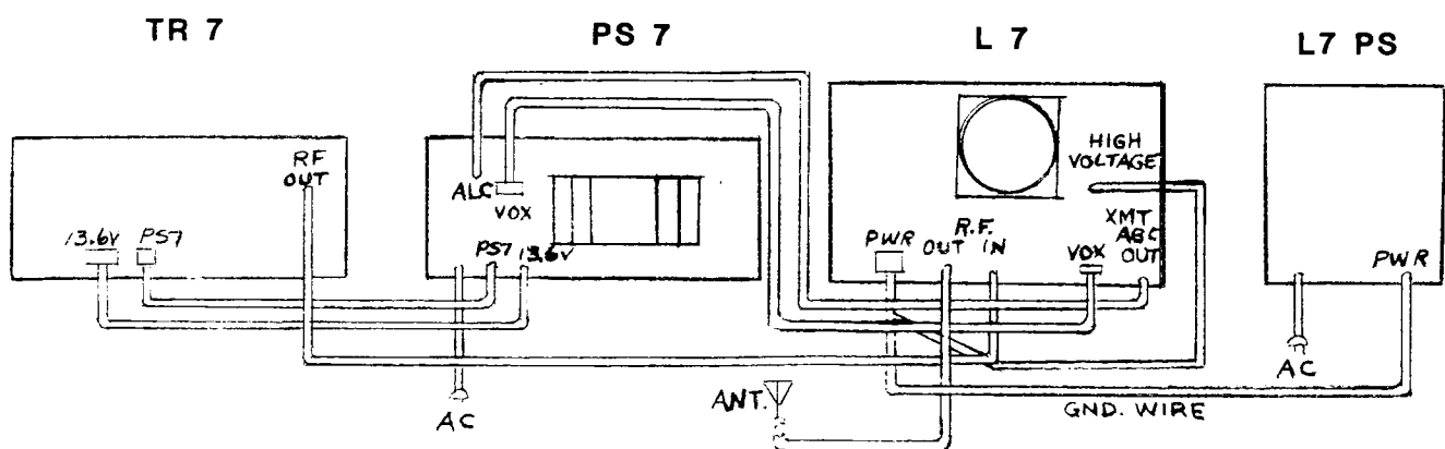
Fig. 2-4 Connecting the PS-7 Power Supply and the R. L. Drake Line of Compatible Exciters
