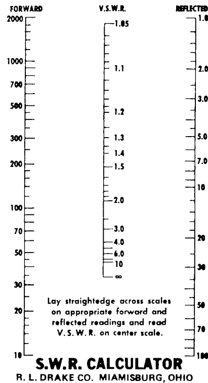
Figure 3-3. SWR Nomograph
